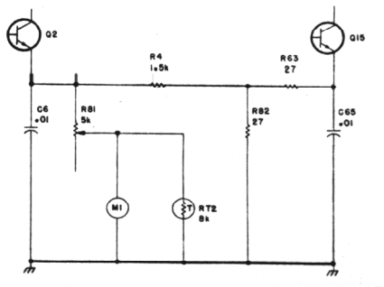
MESSENGER 123A METER CIRCUIT SCHEMATIC DIAGRAM
